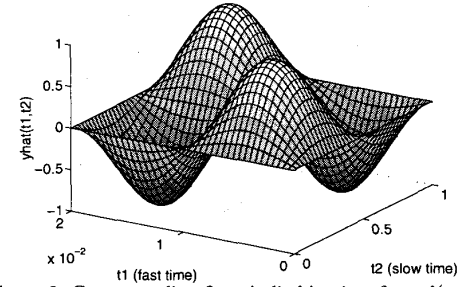
Figure 2: Corresponding 2-periodic bivariate form \hat{y}(t_1, t_2)
