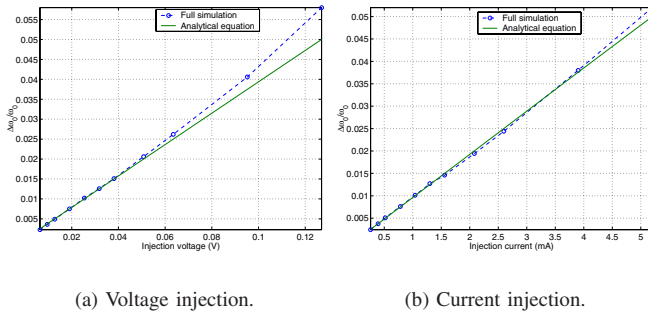
Fig. 4. Maximum locking range of the LC oscillator under different perturbations.
