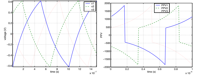
(a) Steady state waveforms of the ring oscillator.
