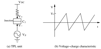
Fig. 5. TPL unit and its voltage-charge characteristic.
