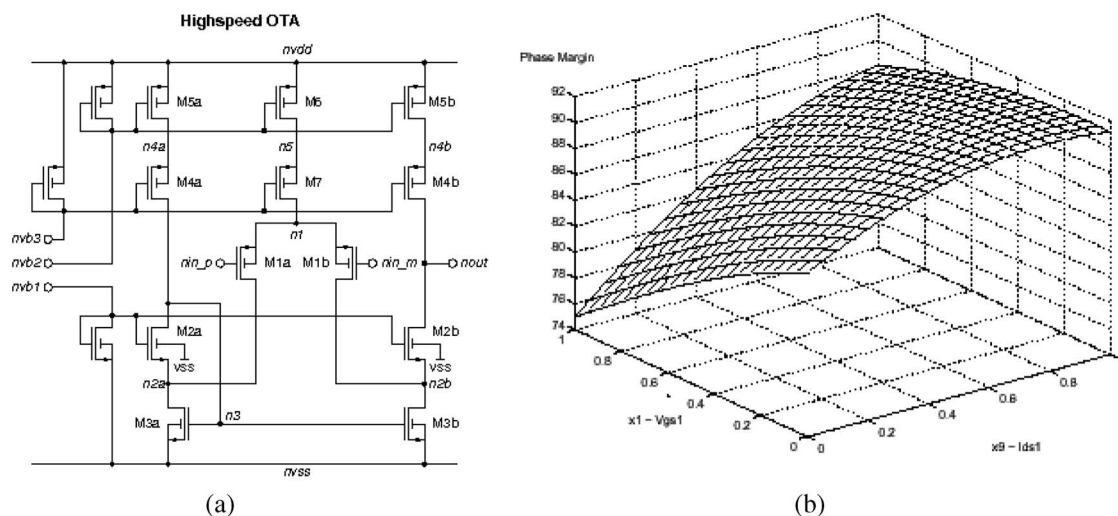
Fig. 19. High-speed CMOS OTA (left) and performance model of phase margin as a function of two design variables (right). Note that this is just a subset of the actual multidimensional parametric performance model.
