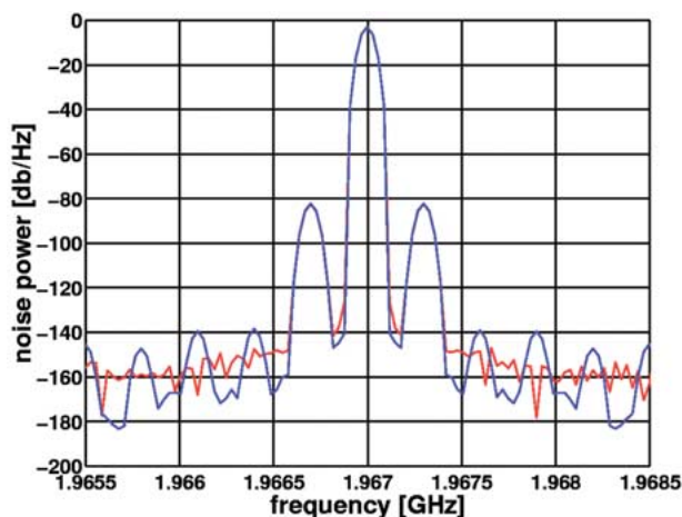
Fig. 18. Frequency response of an extracted behavioral VCO model (blue) compared to the underlying device-level circuit response (red) [8].
