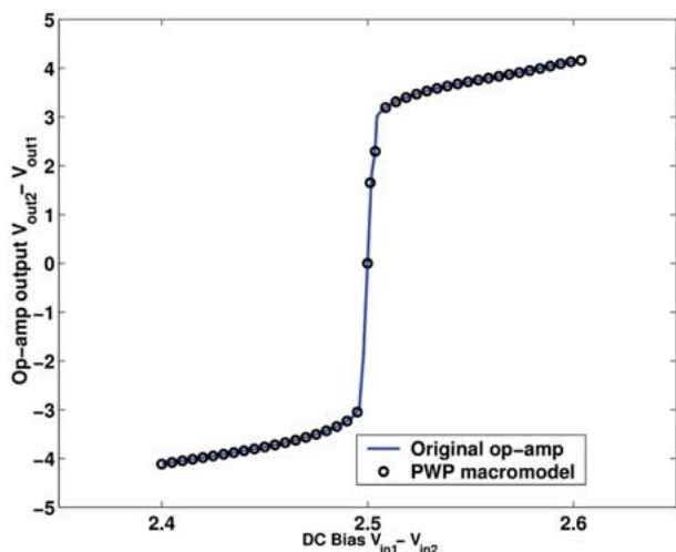
Fig. 7. DC sweep of op-amp from Fig. 6.
