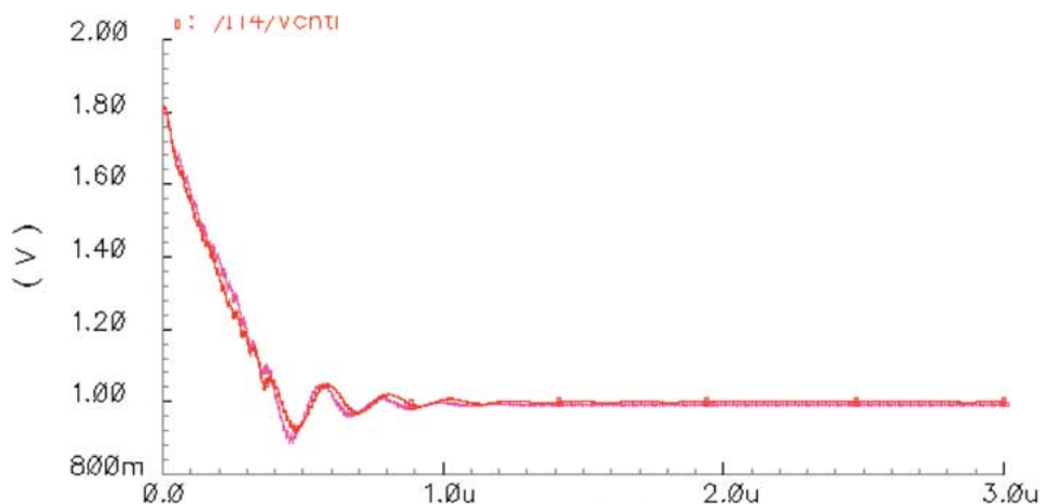
Fig. 28. Comparison plot of the control voltage of the VCO for complete PLL simulation showing both the transistor-level circuit and behavioral model.
