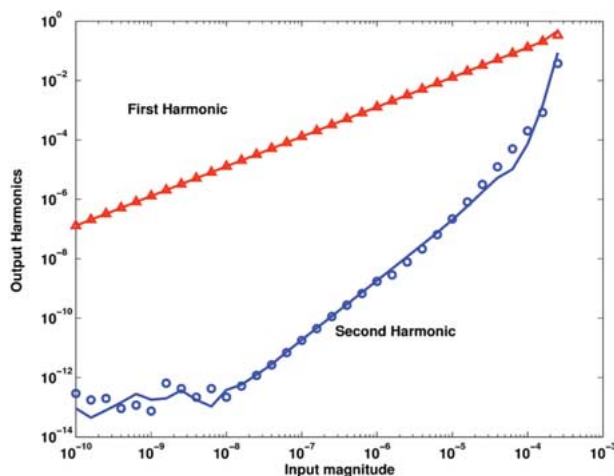
Fig. 9. Harmonic analysis of current-mirror op-amp: full op-amp (solid line) and PWP model (discrete points).
