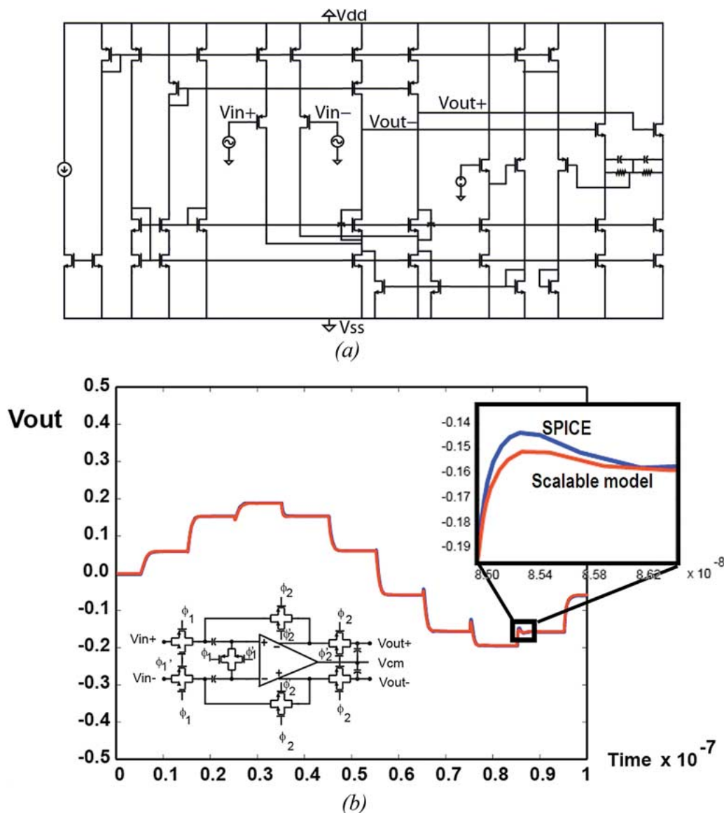
Fig. 11. Example of scalable trajectory model from [85]. (a) CMFB op-amp with 40 MOSFETs, 24 nodes. (b) SPICE versus model accuracy for a scalable trajectory model of CMFB op-amp, hierarchically reinserted into sample-and-hold design.
