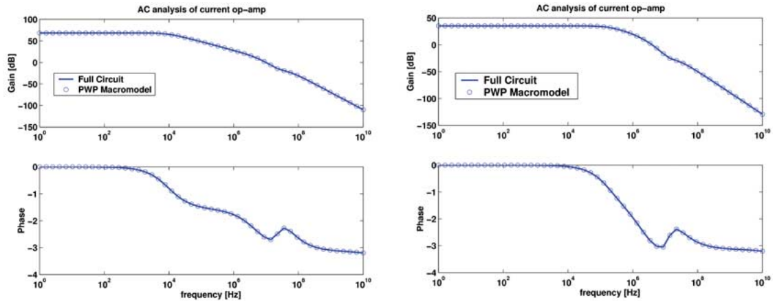
Fig. 8. AC analysis of op-amp from Fig. 6: (left) AC sweep (at common-mode dc bias 2.5 V) and (right) AC sweep (at common-mode dc bias 2.0 V).
