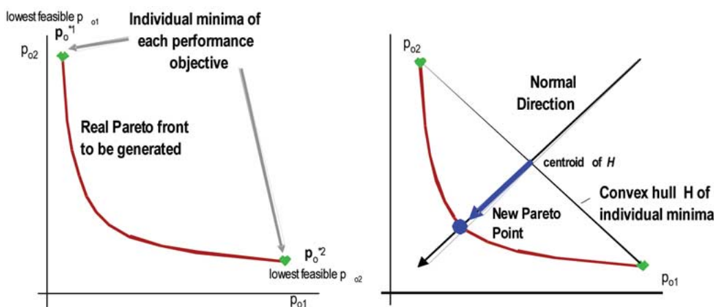
Fig. 24. Illustrating NBI method [96] for tracing Pareto front in two dimensions. From individual minima for two performance objectives (left) the convex hull H (chord, right) of these points is formed, then from the centroid of H a search on the normal is performed to find the new Pareto point.
