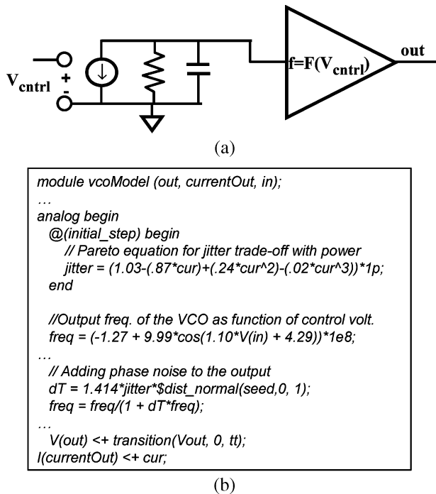
Fig. 27. Overall nonlinear behavior model for VCO: (a) topology for modeling dynamics and nonlinear voltage-to-frequency behavior and (b) verilog-A pseudo-code for adding phase noise from the Pareto front of Fig. 26.
