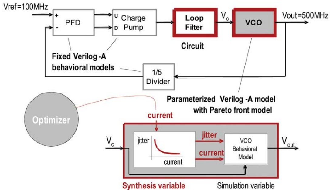
Fig. 25. 2 : 1 PLL hierarchical design scenario from [95].
