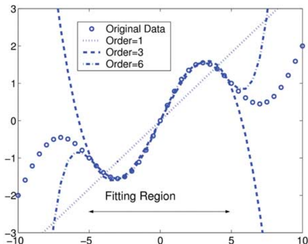
Fig. 5. Limitations of global polynomial approximations.
