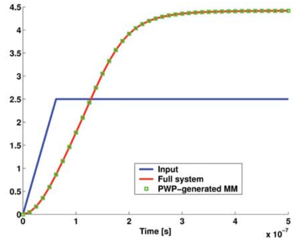
Fig. 10. Transient analysis of current-mirror op-amp with fast step input.
