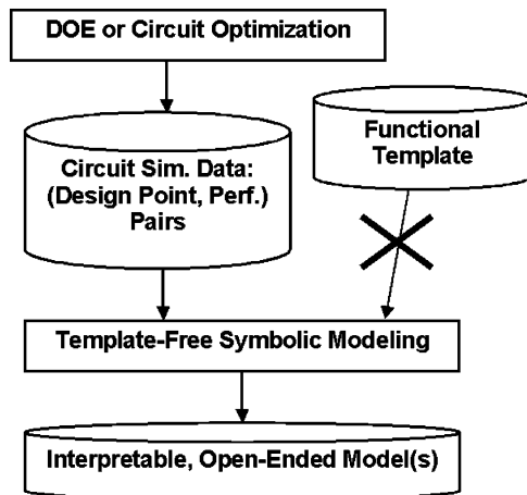
Fig. 20. Flow for template-based and template-free performance modeling.
