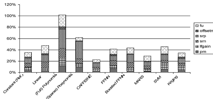
Fig. 23. Comparison of accumulated modeling error for six different performance characteristics of circuit of Fig. 19 for ten different performance modeling methods, starting from the same original set of SPICE data points.
