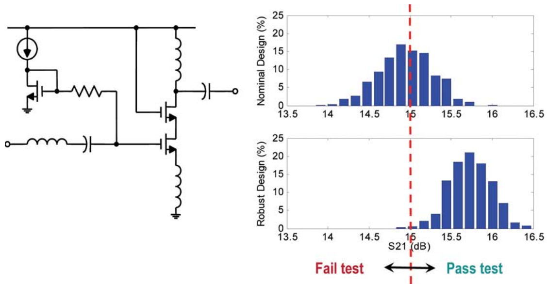
Fig. 31. Applying ROAD methodology for post-nominal statistical robustness optimization on RF LNA in 0.25- \mu\text{m} SiGe process [91].
