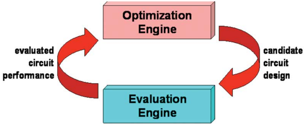
Fig. 16. Basic flow of optimization-based analog circuit sizing.
