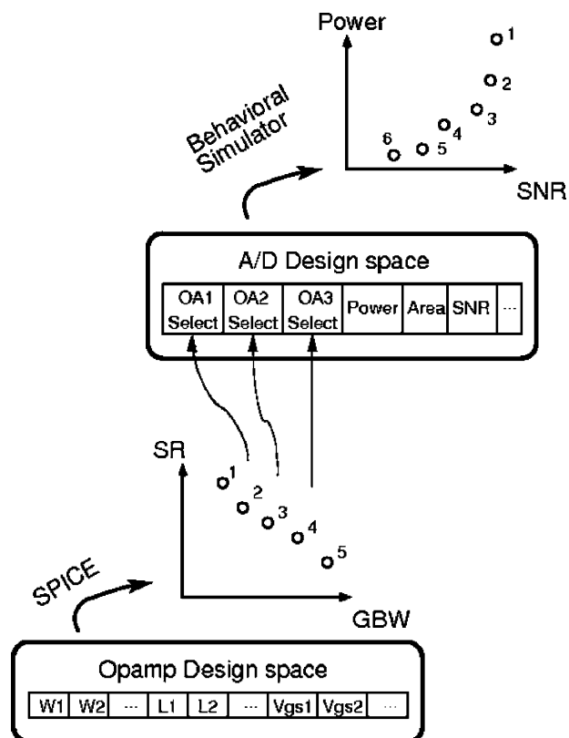
Fig. 29. MOBUs maps design points to performance points via performance simulation as usual. It finds and keeps just the tradeoff via multi-objective optimization. It then propagates tradeoffs upwards where they combine to make the next level's optimal design space.
