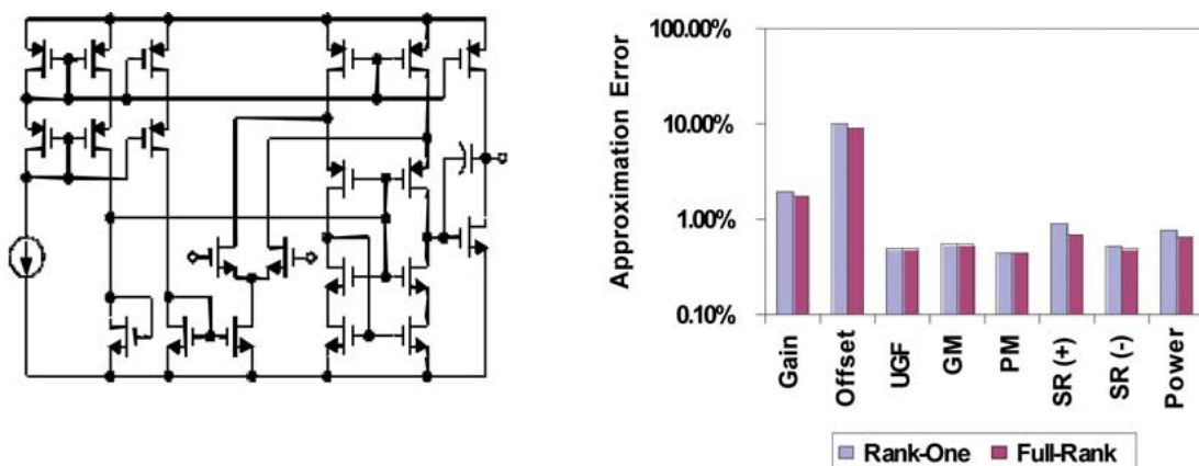
Fig. 21. Applying ROAD [91] projection-based quadratic fitting procedure to 0.25- \mu\text{m} CMOS op-amp. Results show that low-rank approximation strategy is extremely accurate and also reduces fitting complexity from O(N^2) to O(N) .
