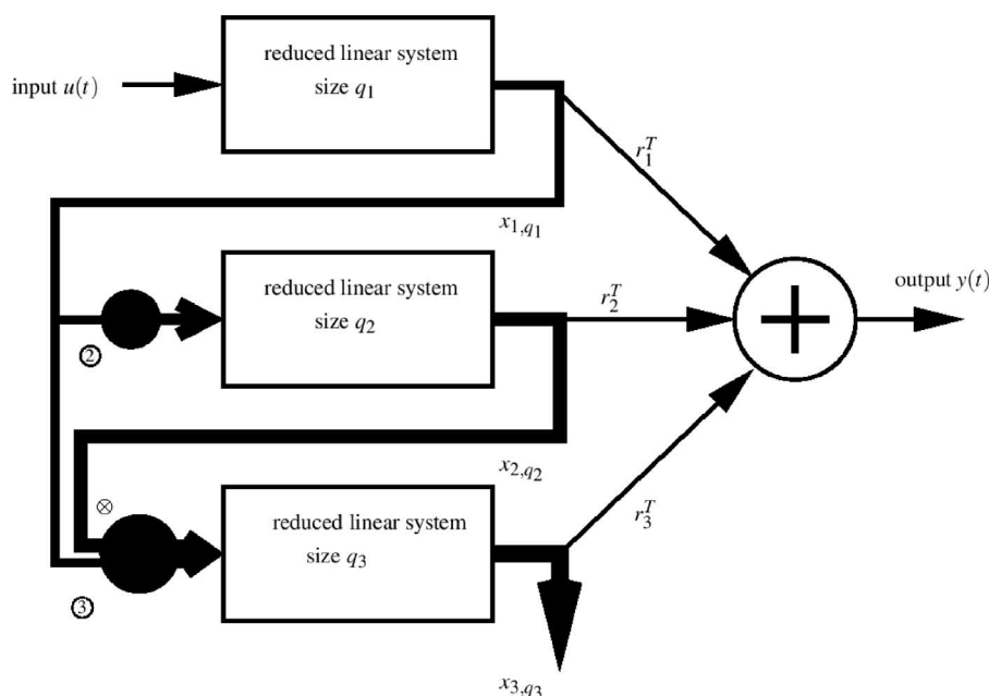
Fig. 3. Overall reduced-order model for a weakly nonlinear system.
