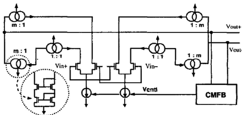
Fig. 6. Current-mirror op-amp with 50 MOSFETs and 39 nodes.
