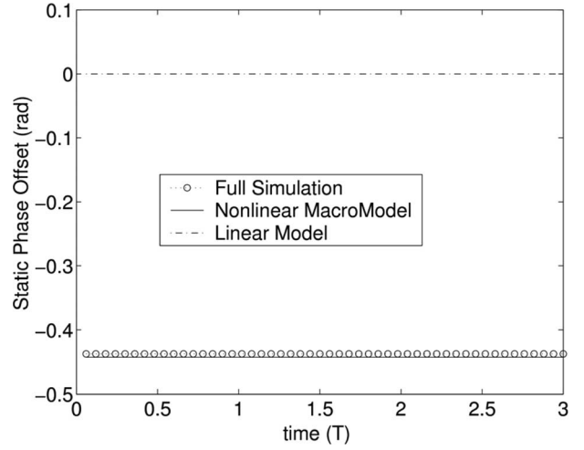
Fig. 13. PLL static phase offset when f_{\text{ref}} = f_0 .
