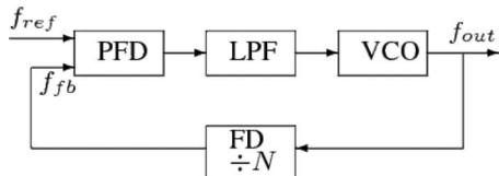
Fig. 12. Functional block diagram of PLL.
