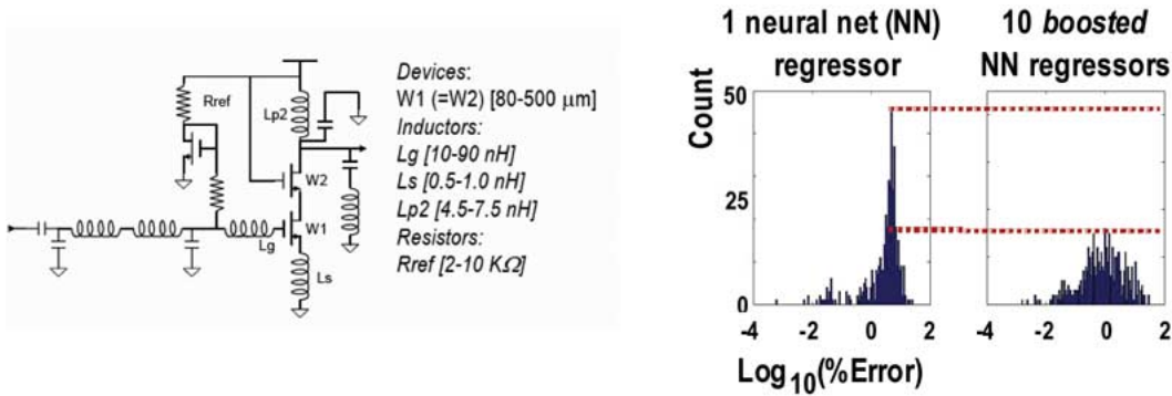
Fig. 22. Example data mining ideas for parametric circuit modeling. RF LNA at left has five designable variables, varying over ranges shown. Histograms at right show fitting error for predicting IIP3, for one simple neural network, and ten boosted neural net based regressors, for fitting 2000 simulated samples of IIP3, across uniform samples of the five design variables. Boosted result makes fewer and much smaller errors [11].
