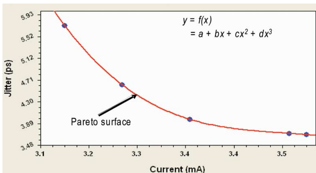
Fig. 26. Extracted jitter versus bias current Pareto front for VCO of Fig. 25.
