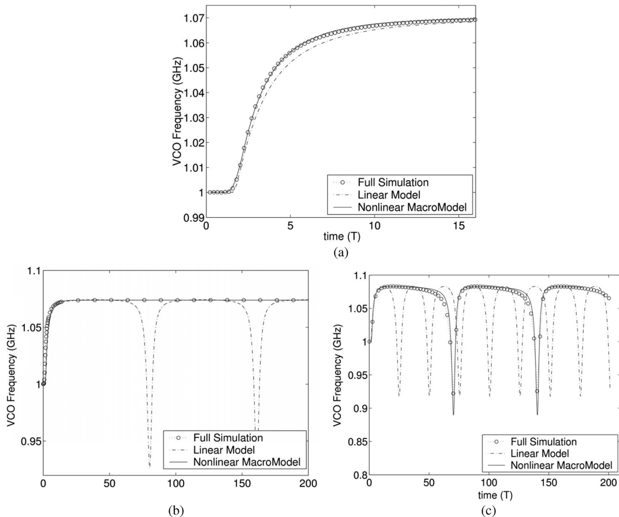
Fig. 14. Step response of PLL model with varying values of f_{\text{ref}} . (a) Response with f_{\text{ref}} = 1.07f_0 . (b) Response with f_{\text{ref}} = 1.074f_0 . (c) Response with f_{\text{ref}} = 1.083f_0 .
