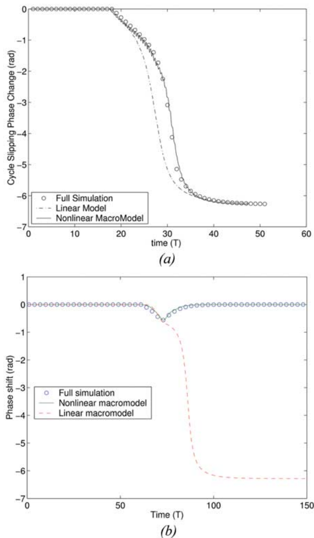
Fig. 15. Cycle slipping of PLL model for different noise amplitudes. (a) PLL cycle slipping, for a noise amplitude of 5 mA. (b) PLL cycle slipping, for a noise amplitude of 3 mA.
