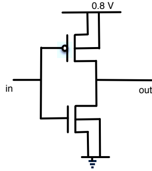
Fig. 5. Inverter circuit.
