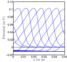
Fig. 11. Several spatial snapshots of the potential propagation in a single dendrite.
