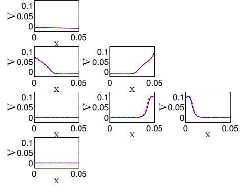
Fig. 18. Comparison of snapshots of potential at t = 0.011 s in a dendritic tree with 7 branches obtained with the H-H model and the ROM. In blue: high-fidelity model, in red: reduced-order model. From top to bottom and then left to right, potential in branches B1, B2, B3, B4, B5, B6 and B7.
