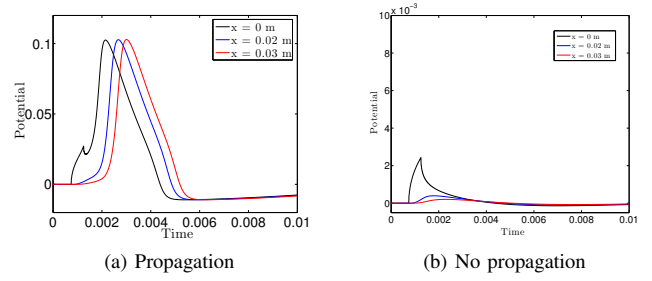
Fig. 12. Transient potential propagation in a dendrite
