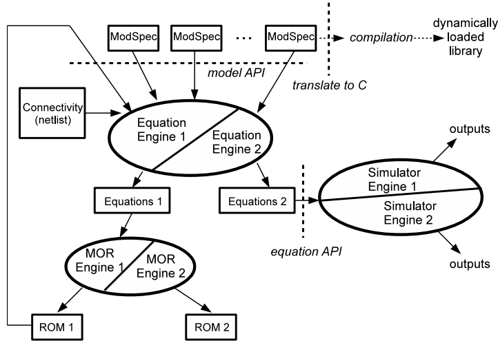
Fig. 4. Schematic description of the model compilation procedure.
