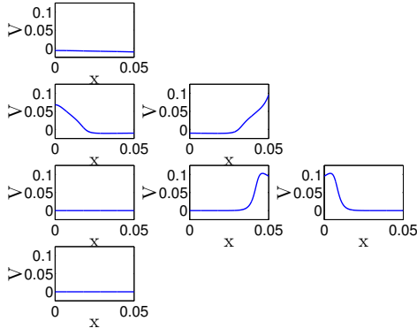
Fig. 15. Spatial snapshot of the action potential propagation at t = 0.011 s in a dendritic tree with 7 branches. From top to bottom and then left to right, potential in branches B1, B2, B3, B4, B5, B6 and B7.
