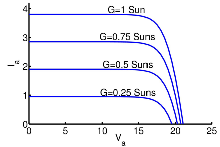
Fig. 8. Solar PV circuit operating at T = 25^\circ\text{C} under various irradiances.
