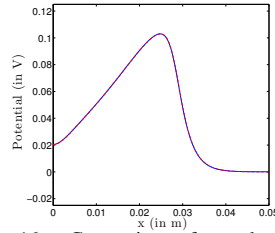
Fig. 16. Comparison of snapshots of potential at t = 0.004 s in a single dendrite obtained with the H-H model and the ROM. In blue: high-fidelity model, in red: reduced-order model.
