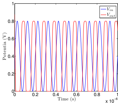
Fig. 6. Inverter circuit output under a sinusoidal input.
