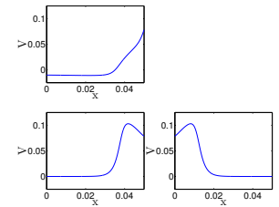
Fig. 14. Spatial snapshot of the action potential propagation at t = 0.007 s in a dendritic tree with 3 branches. From top to bottom and then left to right, potential in branches A1, A2 and A3.
