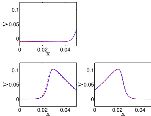
Fig. 17. Comparison of snapshots of potential at t = 0.008 s in a dendritic tree with 3 branches obtained with the H-H model and the ROM. In blue: high-fidelity model, in red: reduced-order model. From top to bottom and then left to right, potential in branches A1, A2 and A3.
