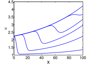
Fig. 9. Snapshots of the evolution of \mathbf{u}(t) at various times t_i with Burger's equation.
