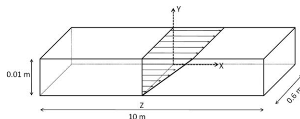
Figure 4. Schematic of the geometry used to model mass transport under oscillatory flow conditions solved by Horn. 9
