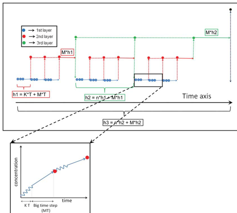
Figure 3. Illustration explaining the telescopic projection technique that was developed by Gear et al. 36
