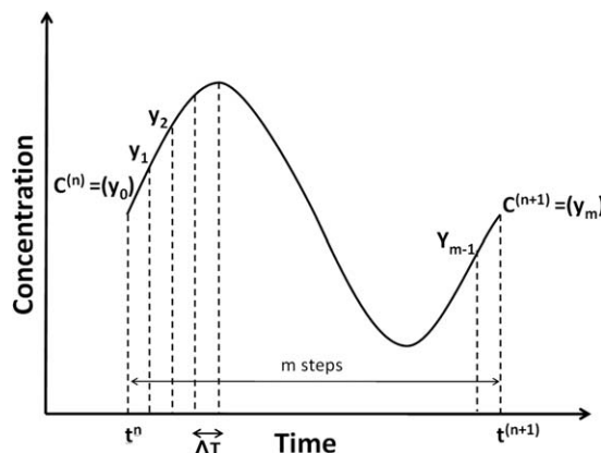
Figure 2. Schematic of the fully implicit envelope-tracking scheme.
