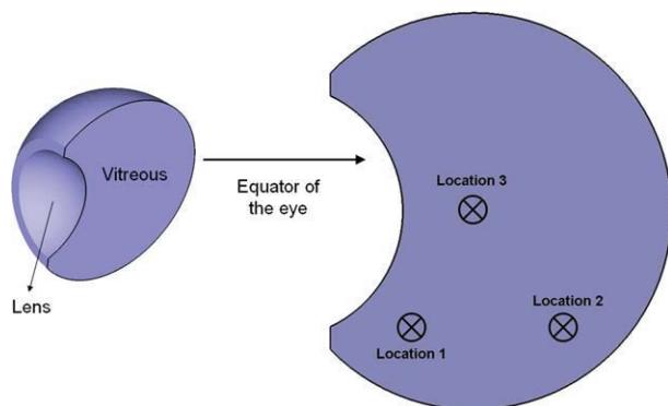
Figure 9. Schematic showing the location of the intravitreal point sources in the equator of the eye.
