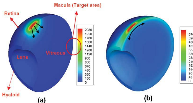
Figure 7. Concentration profile for (a) static and (b) sloshing vitreous after transscleral drug administration.
