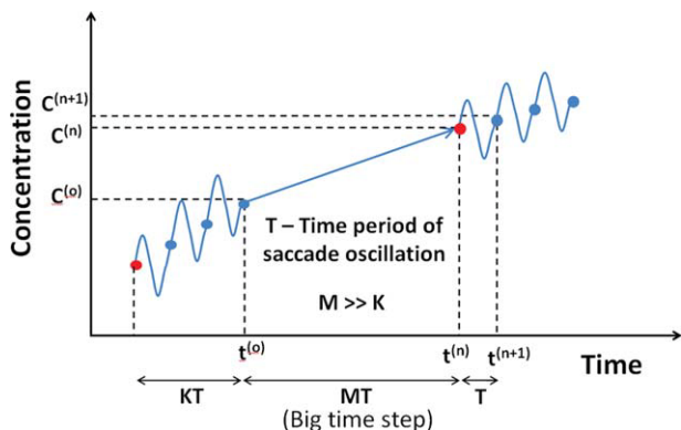
Figure 1. Schematic of the multiscale method proposed by Petzold 22 to bridge the time scales.
