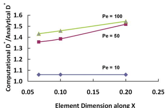
Figure 5. Plot of the effect of mesh refinement on the computed dispersion coefficient for Péclet numbers of 10, 50, and 100 for the test problem.
