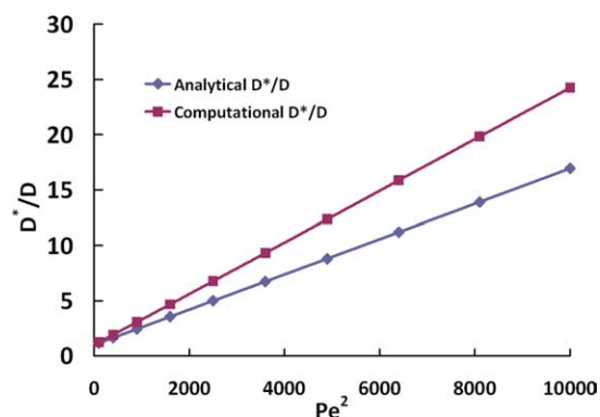
Figure 6. Plot showing the effect of Péclet number (Pe) on the computationally and analytically evaluated dispersion coefficient for the test problem.
