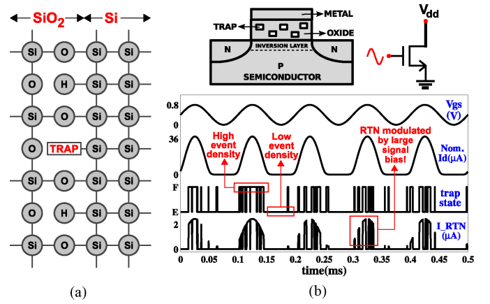
Fig. 4. (a) Dangling bonds at the Si/SiO 2 interface. (b) Trap activity under sinusoidal gate bias, and its modulation by large signal drain current.
