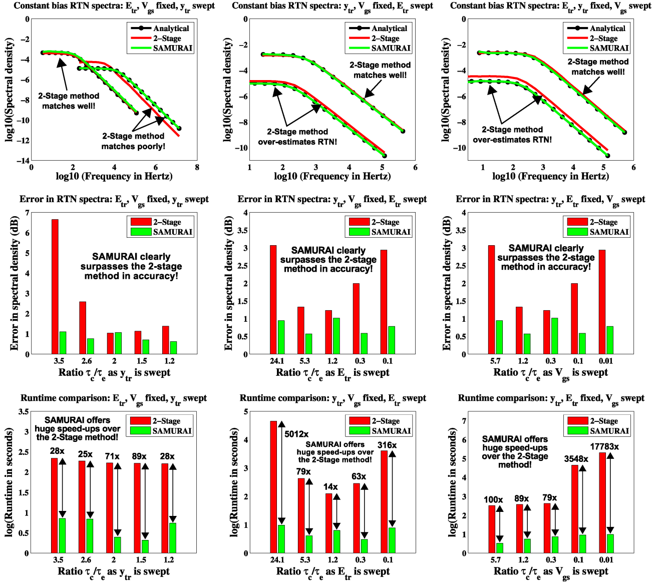
Fig. 10. Comparing SAMURAI against 2-stage RTN generation. The top three plots demonstrate that, even for stationary RTN, the 2-stage method, unlike SAMURAI, does not closely match analytical expressions. The middle three plots show that the 2-stage method can mispredict RTN by several dB, whereas SAMURAI is always within 1 dB of the true spectral density. The bottom three plots show that SAMURAI is much faster than 2-stage RTN generation (note that runtimes are plotted on a logarithmic scale).
